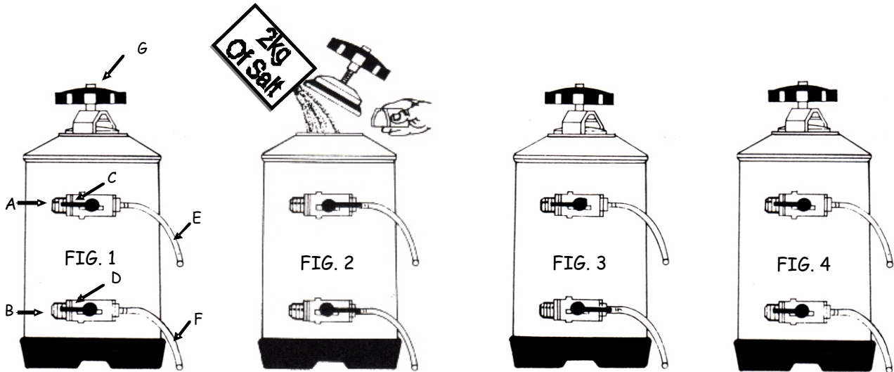
FIG. 1 Softener In Normal Use
